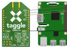
Figure 4 - Corella to R-Pi suggested connection
