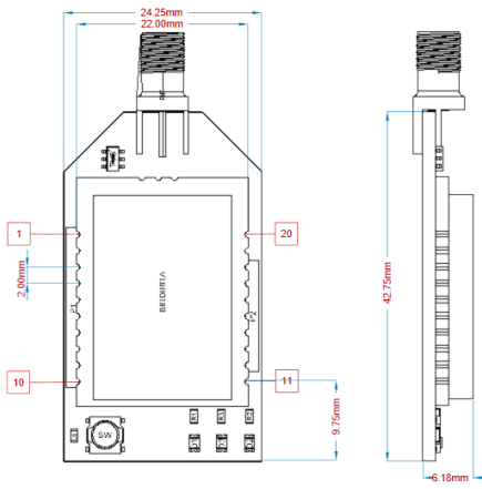
Figure 2 Corella Dimensions
